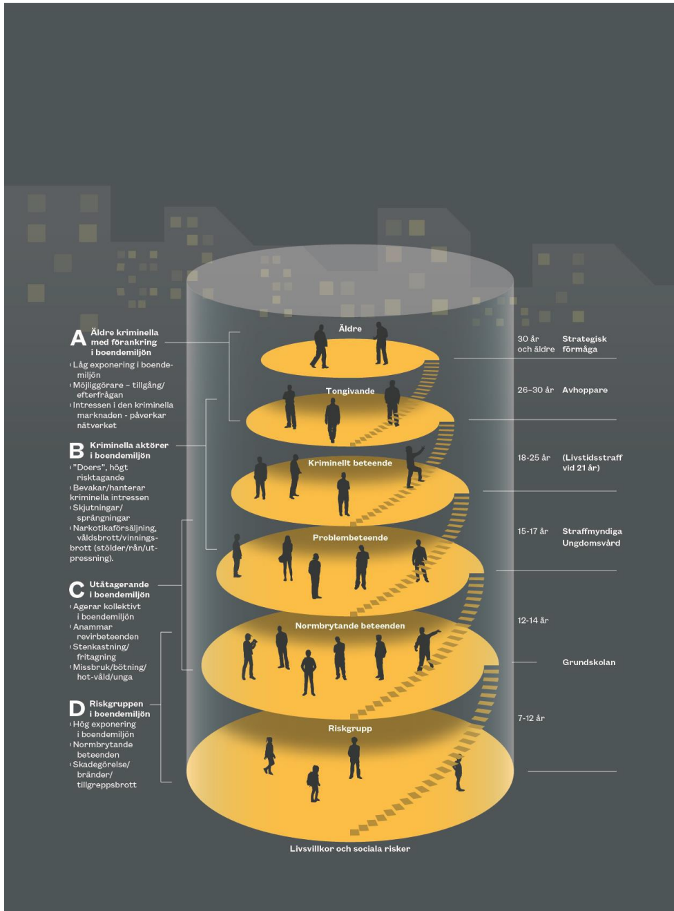
Figur 1. Cylindermodellen
